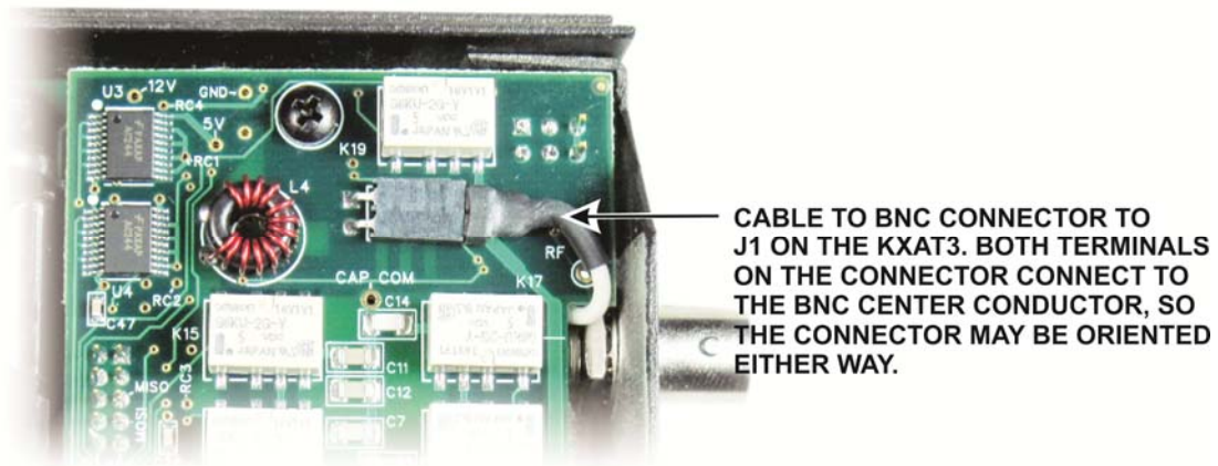
Figure 7. Connecting Antenna Plug to KXAT3 Board.
