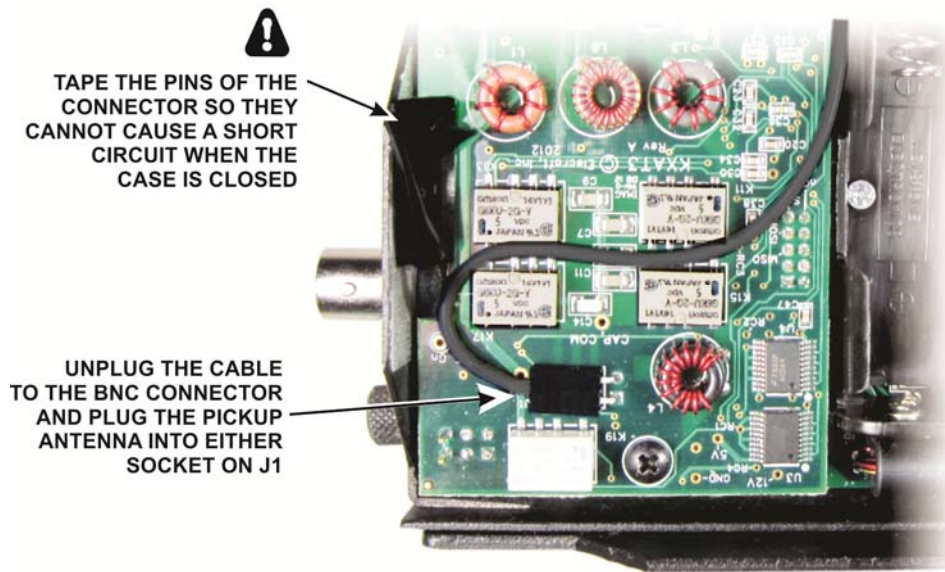
Figure 5. Connecting the Test Antenna to the KX3 Input – With KXAT3.
