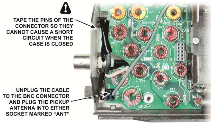
Figure 4. Connecting the Test Antenna to the KX3 Input - No KXAT3.
