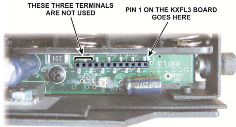
Figure 1. KXFL3 Connector.
