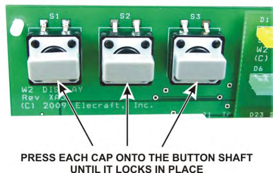
Figure 4. Installing Pushbutton Key Caps.
