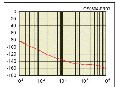
Figure 3 — Worst-case spectral display of the Elecraft K3 transmitter output during composite-noise testing. Power output is 10 W at 14.2 MHz. The carrier, off the left edge of the plot, is not shown. This plot shows composite transmitted noise 100 Hz to 1 MHz from the carrier.
