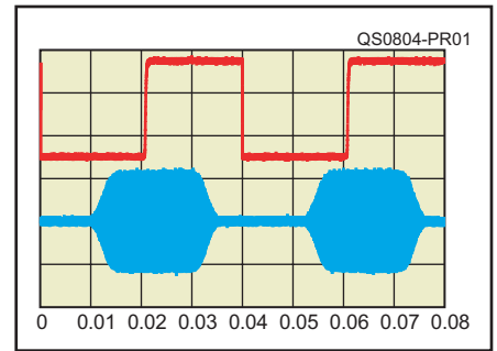
Figure 1 — CW keying waveform for the Elecraft K3/10 showing the first two dits in full-break-in (QSK) mode using external keying. Equivalent keying speed is 60 WPM. The upper trace is the actual key closure; the lower trace is the RF envelope. (Note that the first key closure starts at the left edge of the figure.) Horizontal divisions are 10 ms. The transceiver was being operated at 10 W output on 14.2 MHz.
