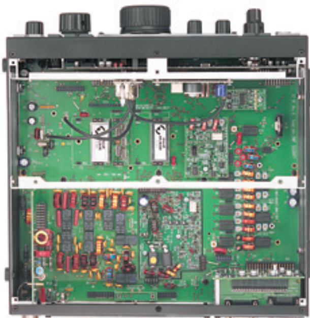
Figure 4 — There's a lot of room inside the K3/10 for options and upgrades such as an antenna tuner, 100 W amplifier or second receiver.
